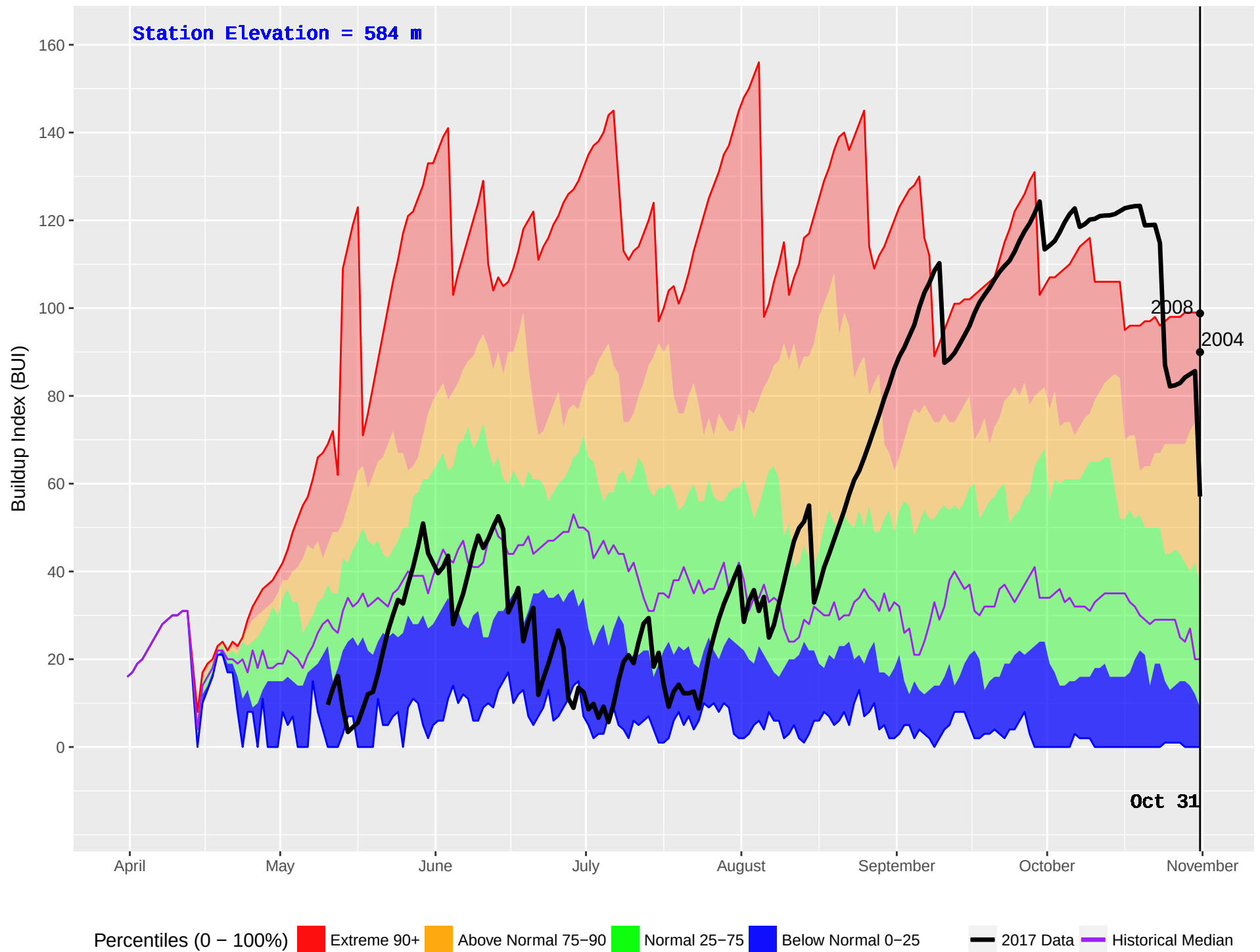
SIERRA (117) : Historical (1981–2016) and Current (2017) Noon Buildup Index (BUI)
