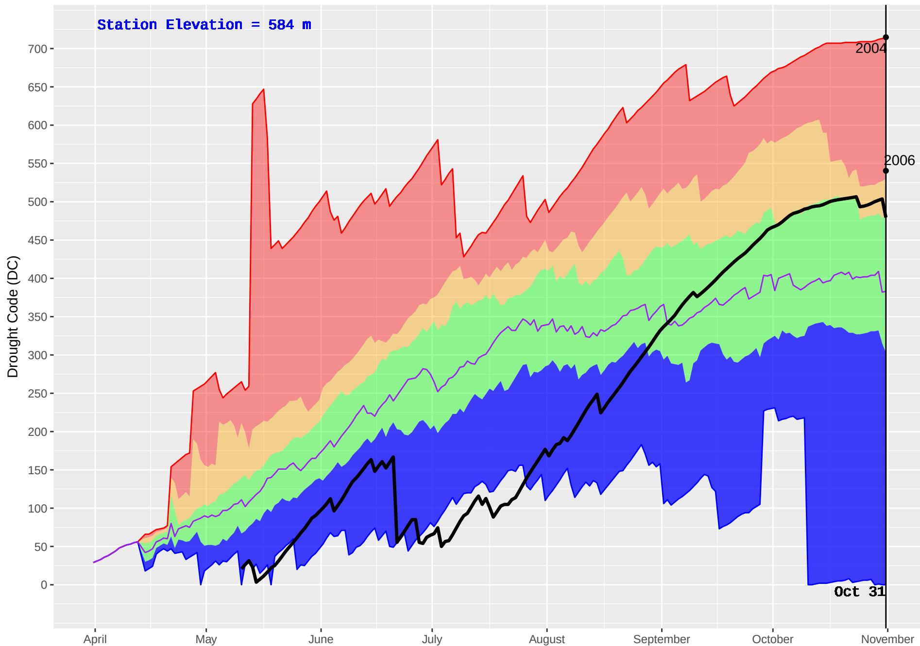
SIERRA (117) : Historical (1981–2016) and Current (2017) Noon Drought Code (DC)
